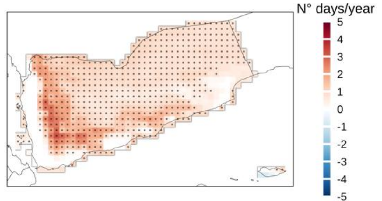
Change (days/year) in annual count of days with TX (daily maximum) > 25^{\circ}\text{C}
