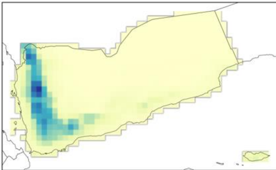
Annual count of days with PRCP <1mm
