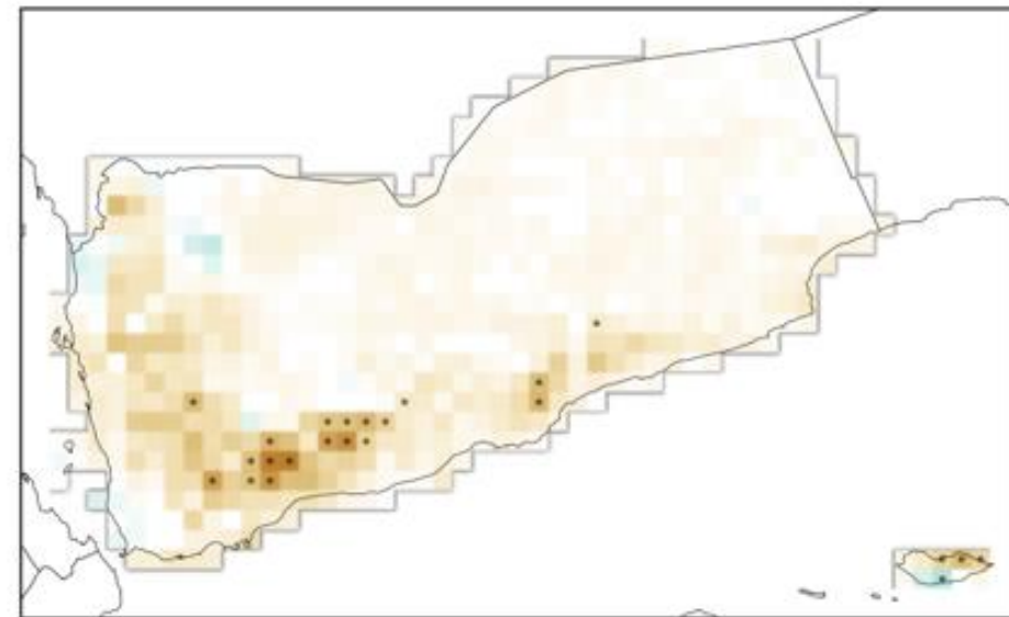
Change (days/year) in annual count of days with PRCP <1mm
