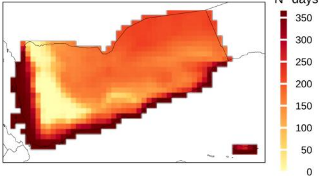
Annual count of days with TN (daily minimum) > 20^{\circ}\text{C}
