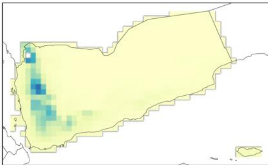
Total annual precipitation (mm)
