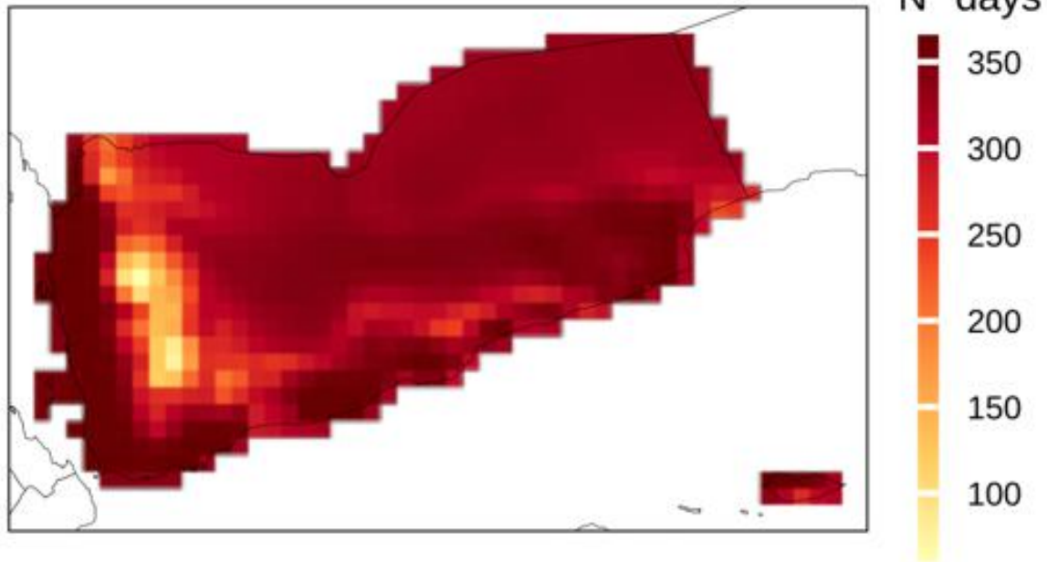
Annual count of days with TX (daily maximum) > 25^{\circ}\text{C}
