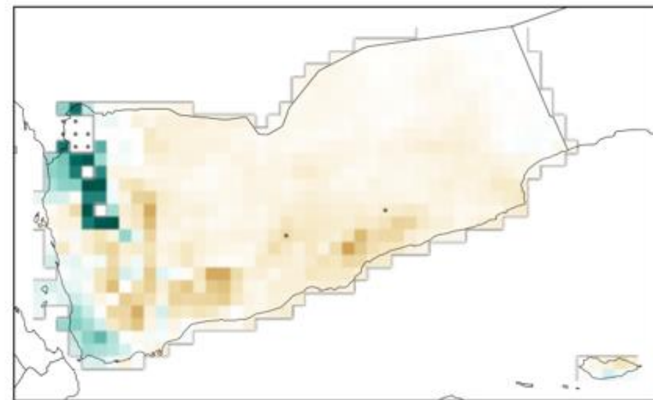
Change (mm/year) in total annual precipitation
