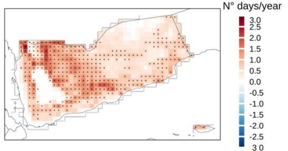
Change (days/year) in annual count of days with TN (daily minimum) > 20^{\circ}\text{C}
